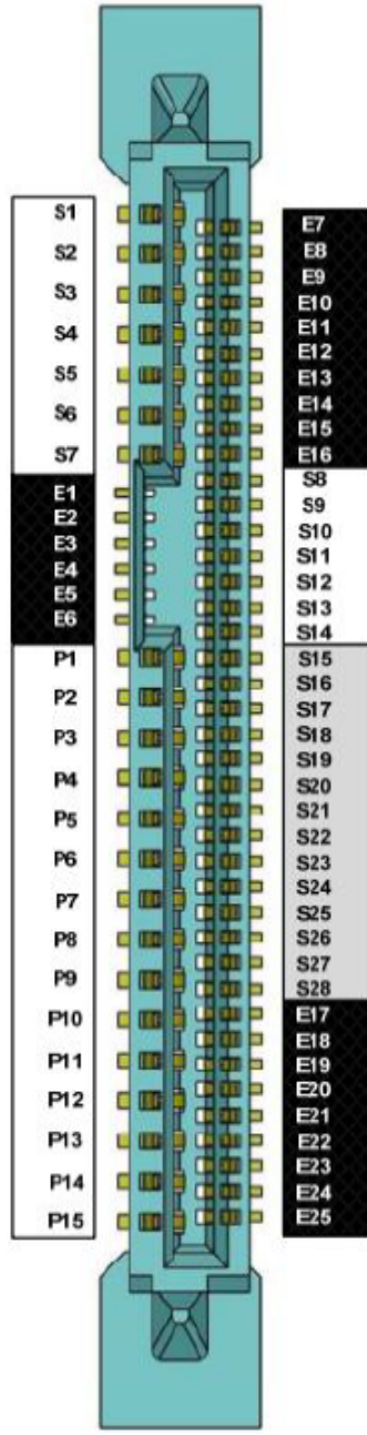
SFF-8639 U.2 pinout (Input)
