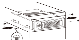
M3*4 Screw
