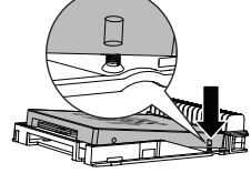
Press down the front of the drive to align with the built-in screws on the tray. Make sure the screws fit into the drive securely.
