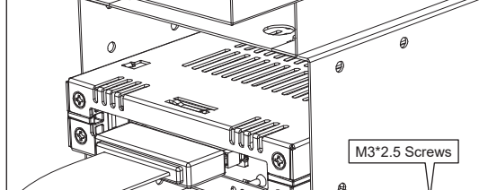
4-1. Insert the MB741V4P-B into external 3.5" bay and use the included 4 x M3*2.5 screws to secure the device onto the bay.
